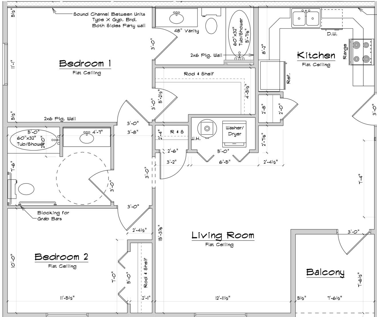
AUBURN HILLS - TWO BEDROOM - 1144 SQ FT
